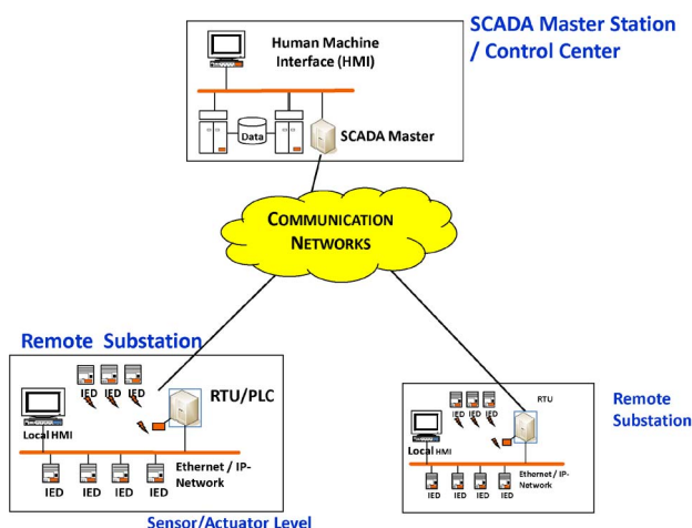
Fig. 1. A power grid SCADA system.
