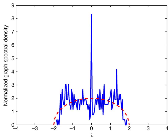
Fig. 5. The normalized graph spectral density of the sample 396-node MV distribution network, \bar{\rho}(\lambda) vs. \lambda ; the dotted line of semicircle represents the graph spectral density of random graph networks.
